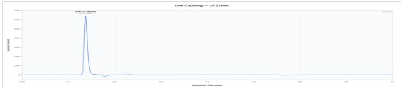
GHK-Cu 50mg - GHKCU-08-24-26: UV Chromatogram
