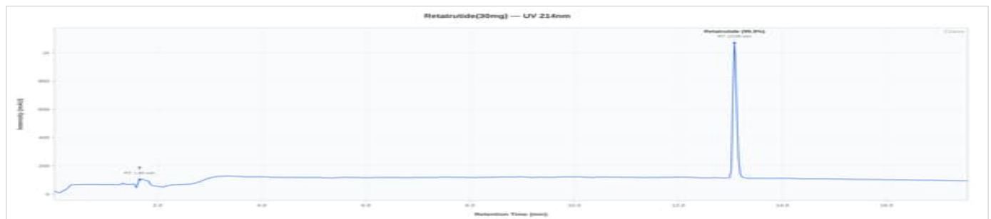
PBL-R3 30mg - G3RT30-07: UV Chromatogram
