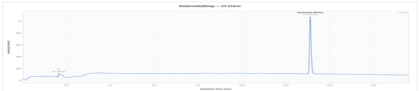
PBL-R3 30mg - G3RT30-03: UV Chromatogram
