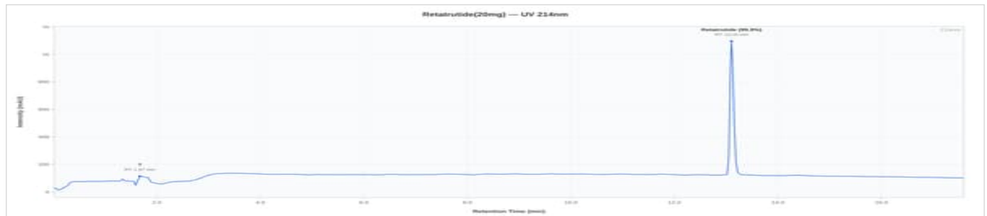
PBL-R3 20mg - G3RT20-03: UV Chromatogram
