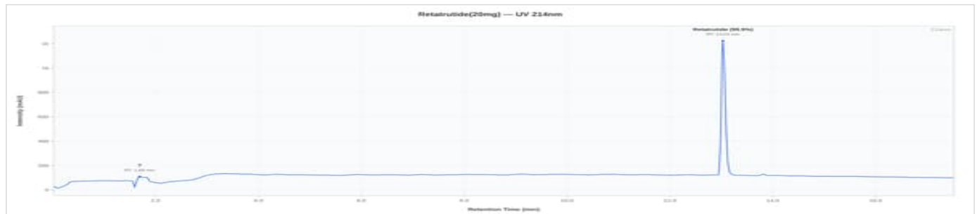
PBL-R3 20mg - G3RT20-02: UV Chromatogram
