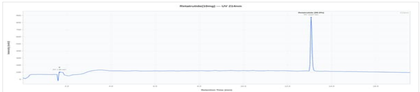
PBL-R3 10mg - G3RT10-02: UV Chromatogram
