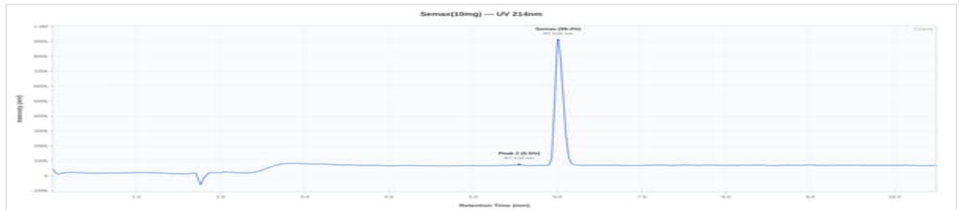
Semax 10mg - PX36826: UV Chromatogram
