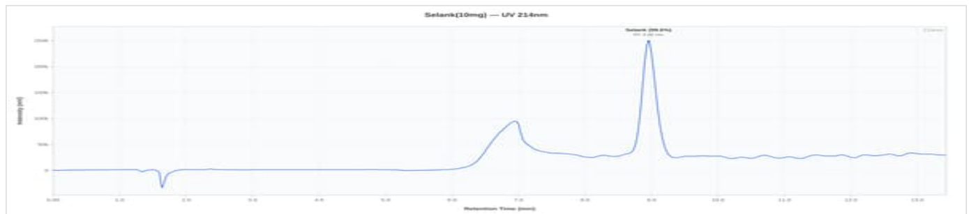
Selank 10mg - PX35826: UV Chromatogram
