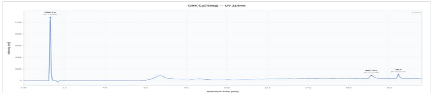
GLOW 70mg - PX10826: UV Chromatogram
