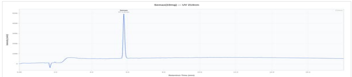
Semax 10mg - SM1026246JP: UV Chromatogram
