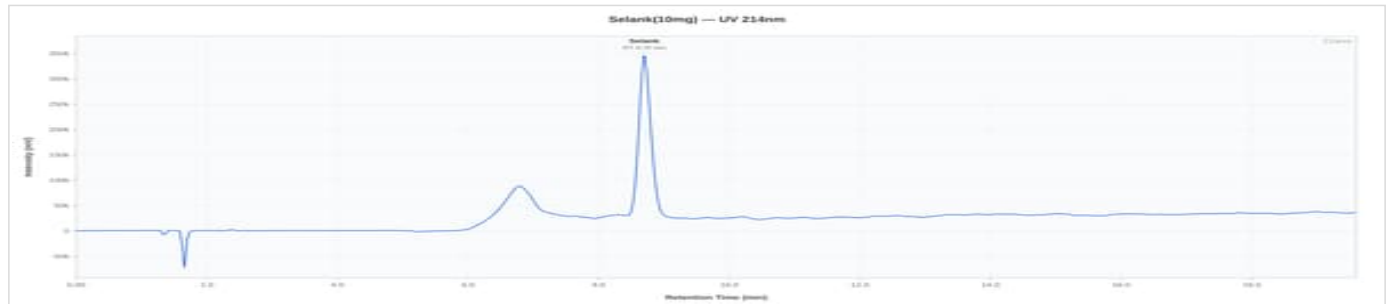
Selank 10mg - SL1026246JP: UV Chromatogram
