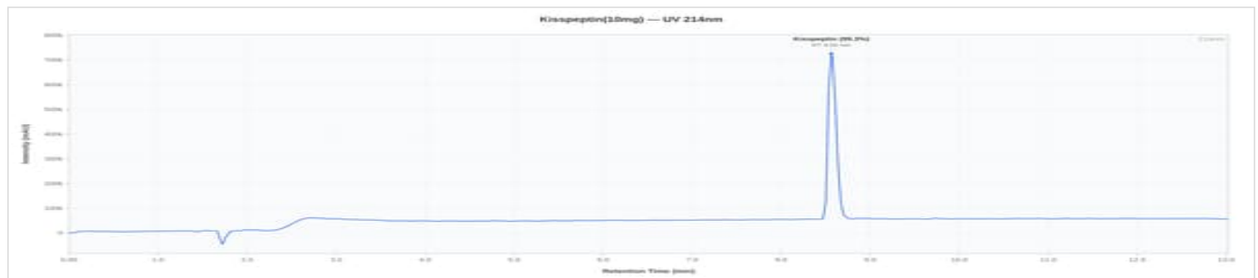
Kisspeptin 10mg - OS-2026-8274: UV Chromatogram
