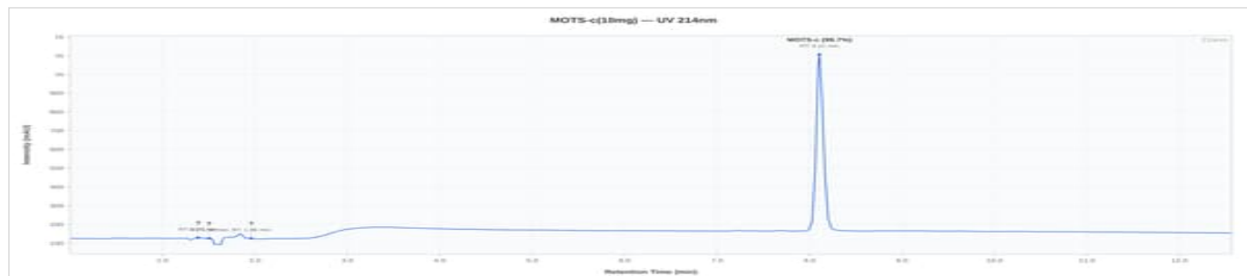
MOTS-C 10mg - MPMC005: UV Chromatogram
