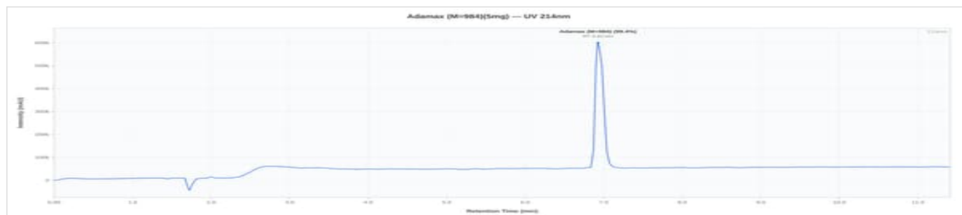
Adamax 5mg - HR-2026-6715: UV Chromatogram
