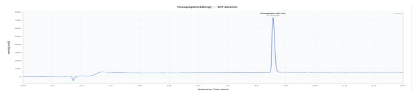
Kisspeptin 10mg - HR-2026-3156: UV Chromatogram
