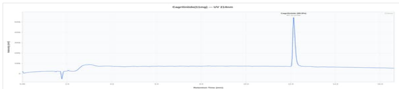
Cagrilintide 11mg - 26-U5-YCT / CAG100502-1: UV Chromatogram
