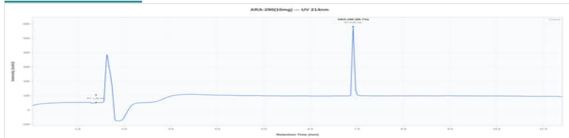
ARA-290 10mg - 26-L5-BST / 10RA050126-1: UV Chromatogram
