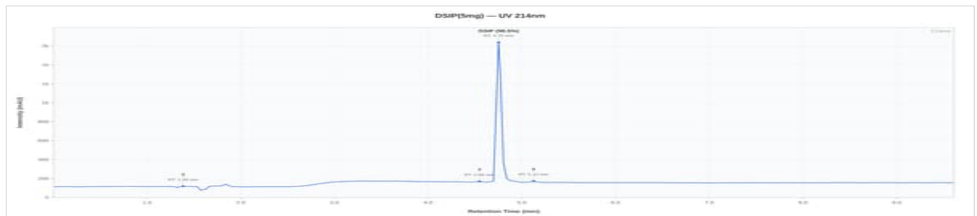
DSIP 5mg - 5DS626: UV Chromatogram
